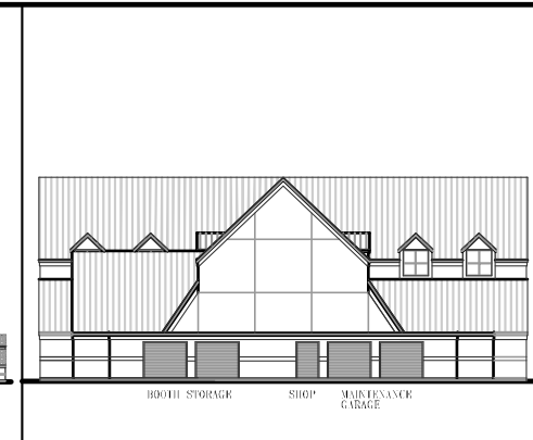
SOUTH ELEVATION
